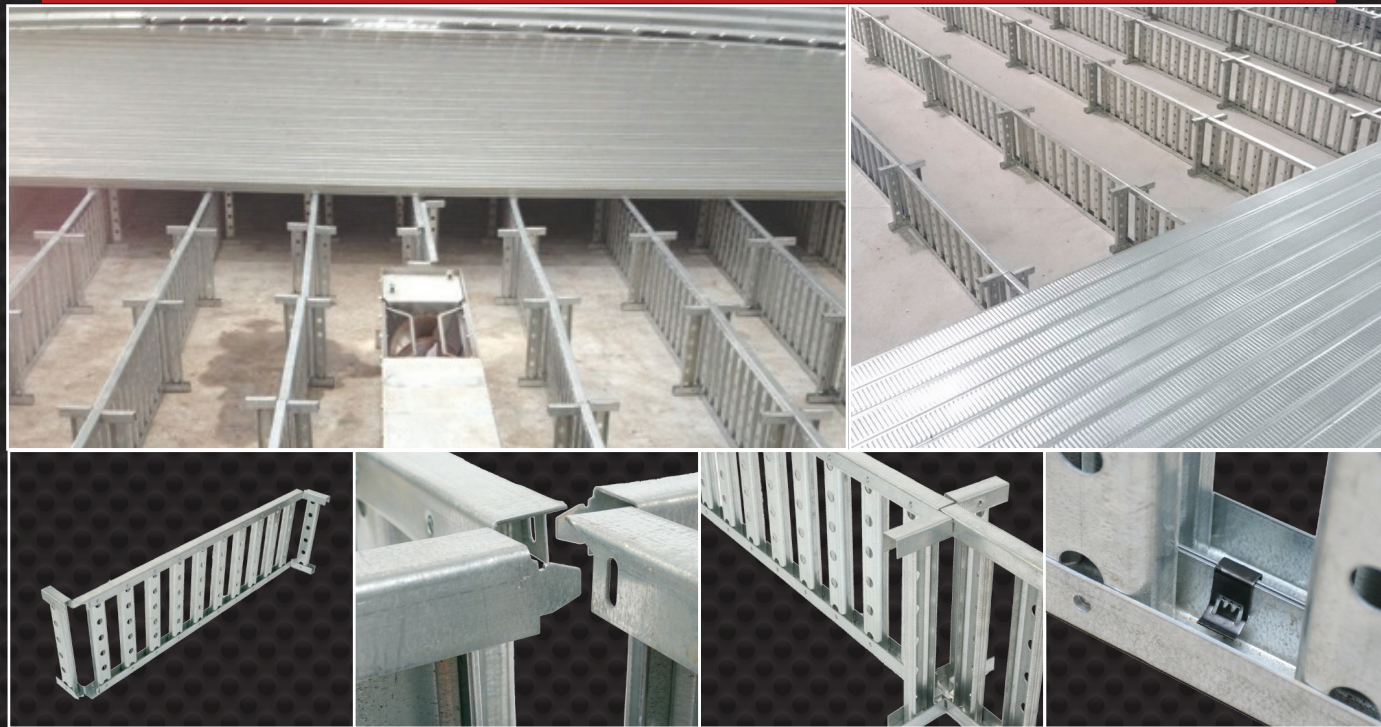
SYNTRINO Ladder Support
