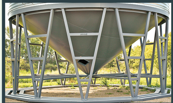
Assie Engineered cones to 27' dia.
