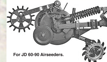
The 2966 Residue Manager from YETTER Clears residue from the front of the opener blade for improved seed disc opener performance. Places residue just to the side of the row rather than tossing it into adjoining rows. Heavy duty pivot allows the wheel to float over the soil surface.
